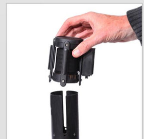
Step 3: Loosen the cassette retaining screws and slide out the cassette
